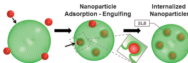
Figure 1. Scheme depicting the mechanism of NP internalization. Hydrophilic NPs adsorb to the lipid are wrapped and finally internalized into the fluid liposomes, thereby forming supported lipid bilayer (SLB) NPs (the inset depicts the process of invagination).
